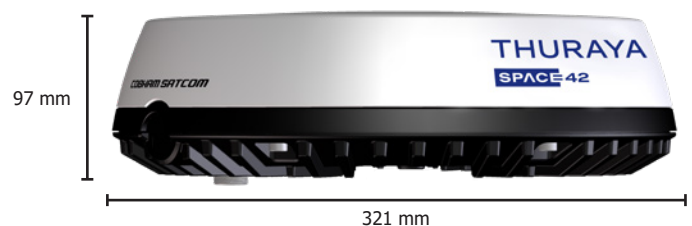
Orion NEO Antenna Dimensions
