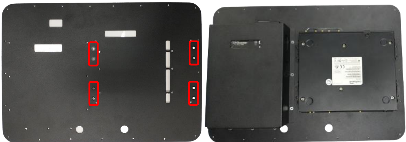
Figure 7: For AER2200 router, fasten the router to the cover plate using PTA0399-TL screws.
