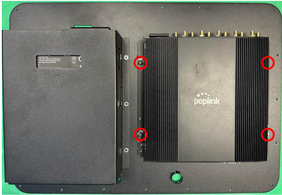
Figure 11: For Peplink MAX BR2 Pro 5G router, fasten the router to the cover plate using PTA0399-TL screws.
