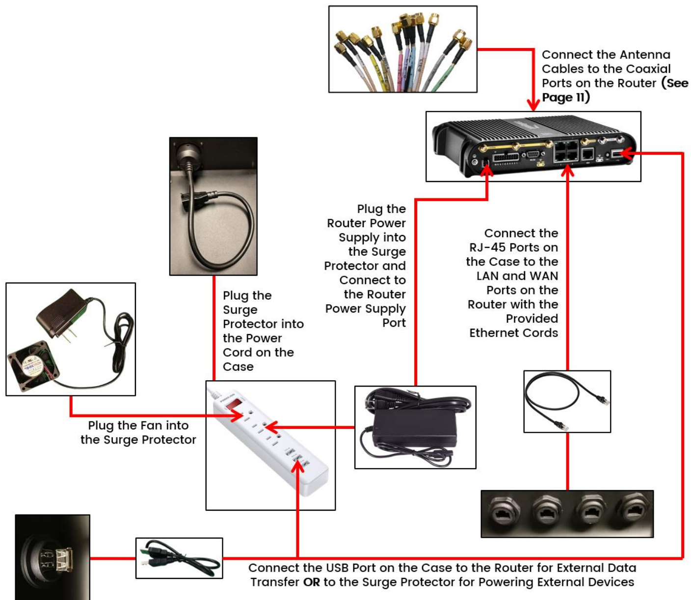
Figure 13: Connection Diagram for Bloodhound L
