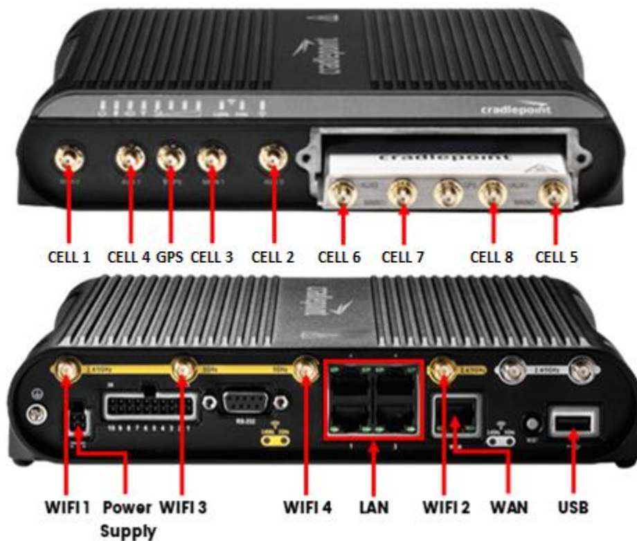
Figure 15: Cradlepoint IBR1700 Connections
