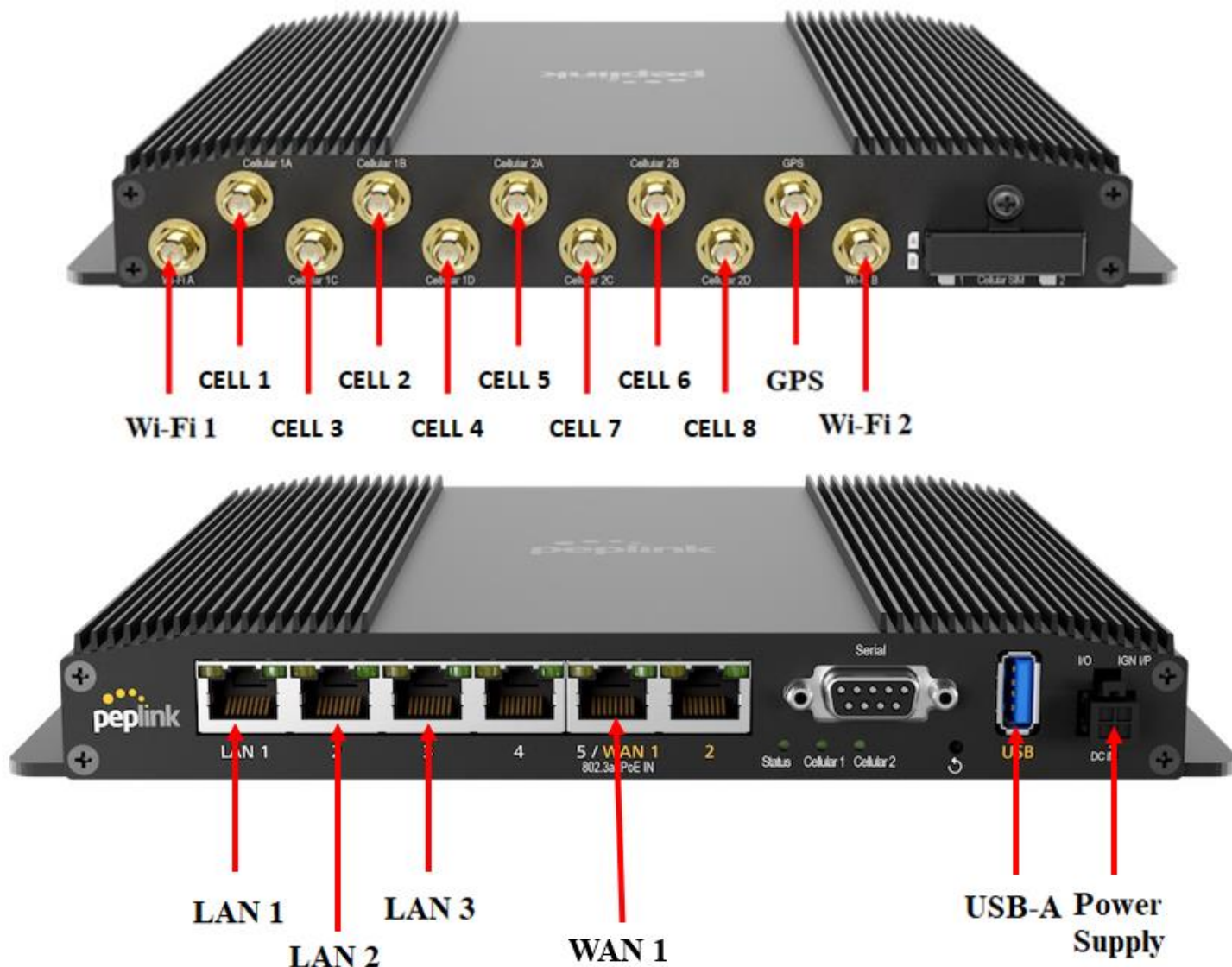
Figure 17: Peplink MAX BR2 Pro 5G Connections – 3 LAN, 1 WAN
