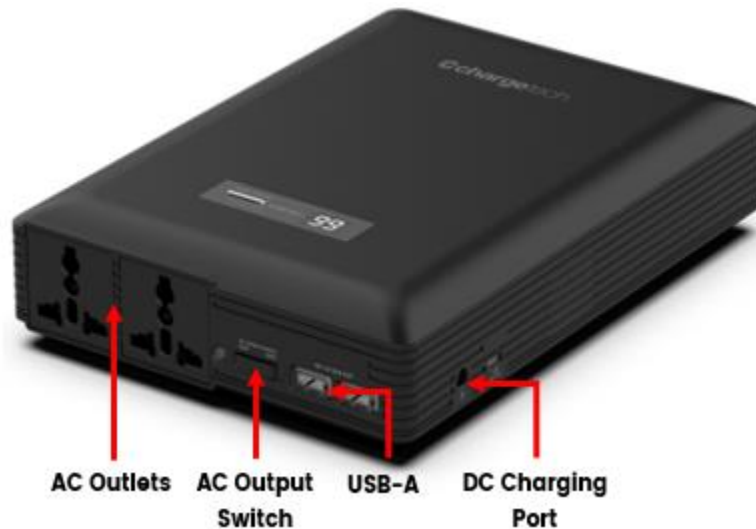
Figure 19: ChargeTech 54K Battery Pack Connections. (Bloodhound G)
