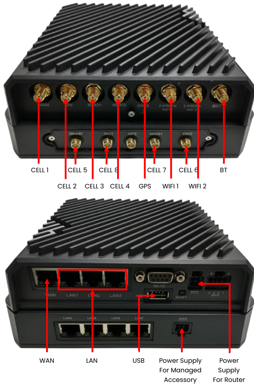
Figure 16: Cradlepoint R1900 Connections
