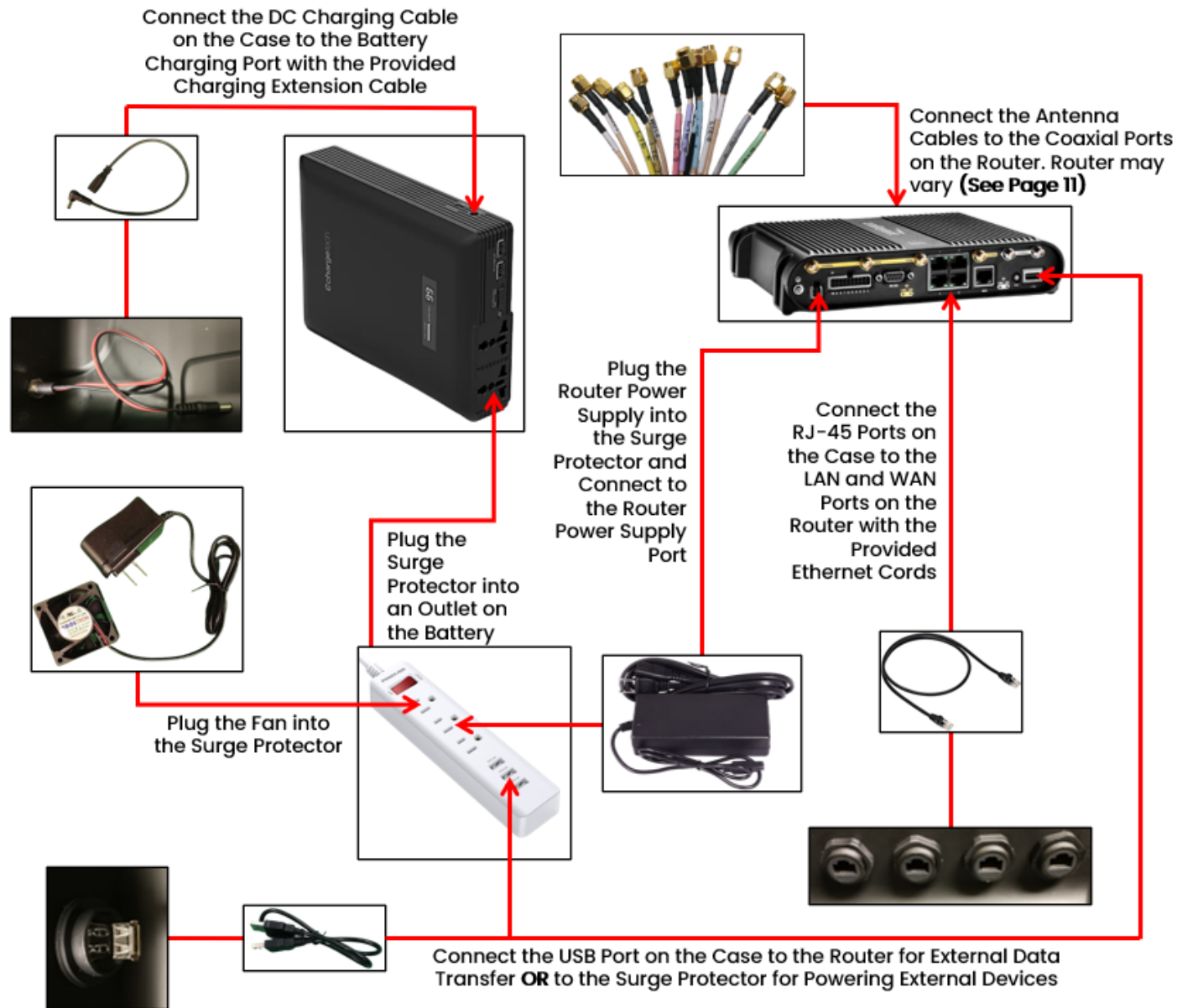
Figure 12: Connection Diagram for Bloodhound G & G1
