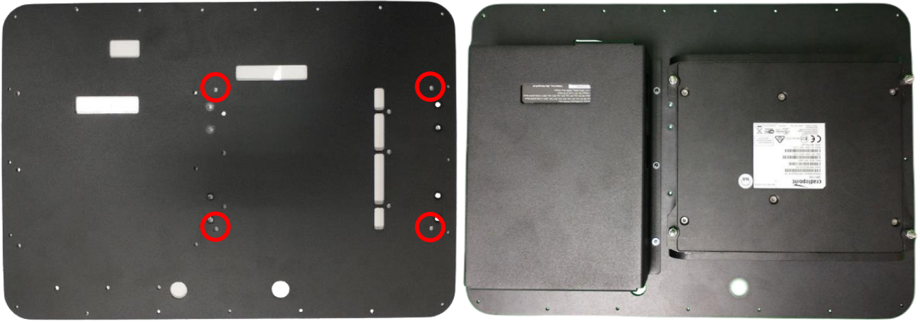
Figure 8: For IBR1700 router, fasten the router to the cover plate using PTA0579 screws, PTA0140 washers, PTA0844 lock washers, and PTA0408 nuts.
