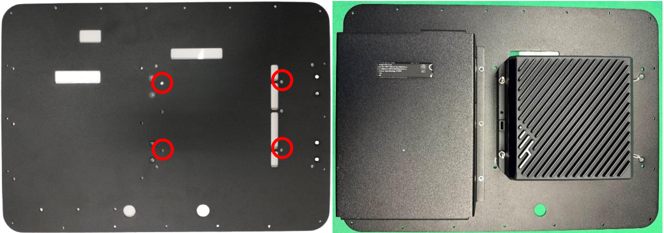
Figure 10: For R1900 router and MX-30 Managed Accessory, fasten the router to the cover plate using PTA0579 screws, PTA0140 washers, PTA0844 lock washers, and PTA0408 nuts.
