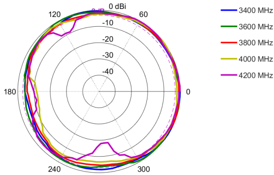
Azimuth: 3400 – 4200 MHz
