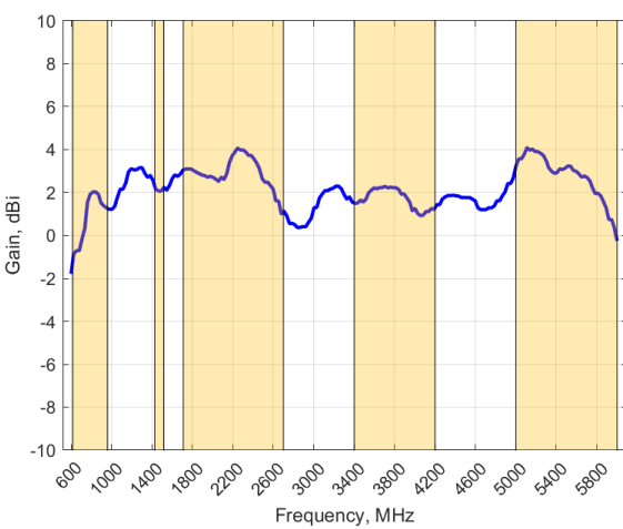
GAIN (EXCLUDING CABLE LOSS): Cellular Horizontal
