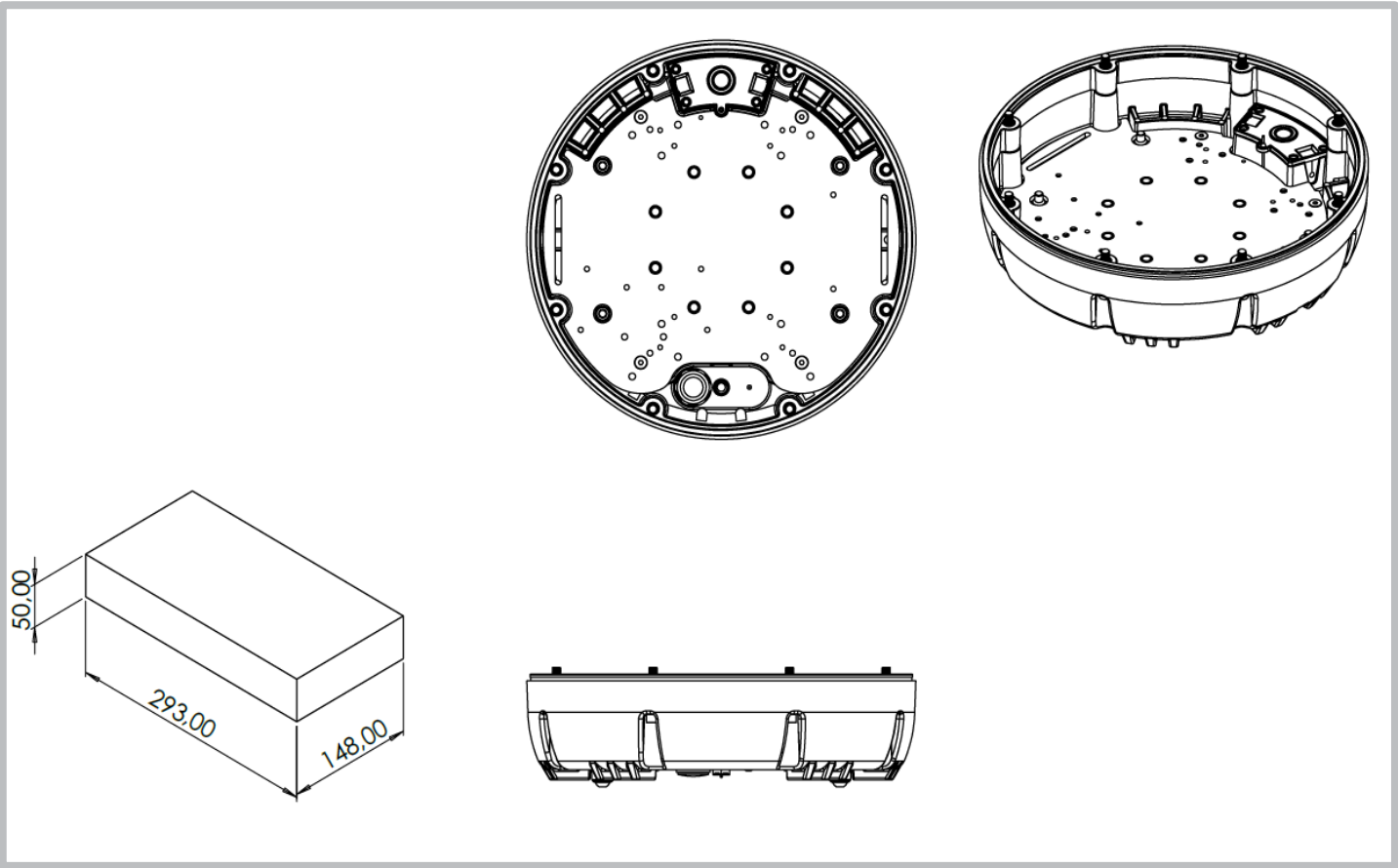
SWIRL Base Available Router Space (Horizontal)
