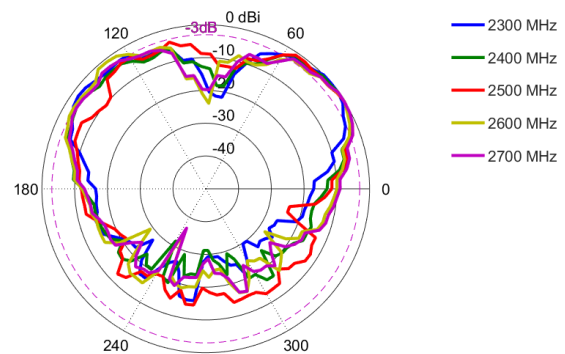
Elevation: 2300 – 2700 MHz
