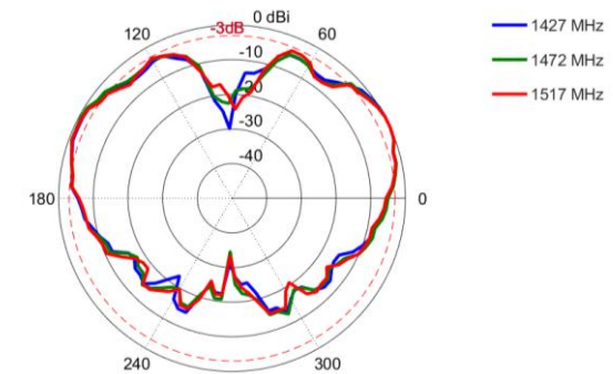
Elevation: 1427 – 1517 MHz
