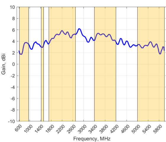
GAIN (EXCLUDING CABLE LOSS): Cellular Vertical
