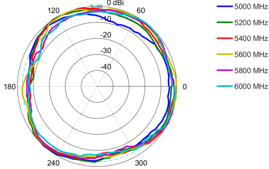
Azimuth: 5000 – 6000 MHz
