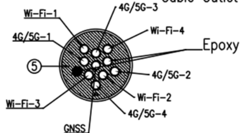
Bottom Thread View Cable Outlet
