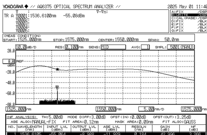
Fig.1: Signal amplification at 1536.61nm @ Pin -55dBm
