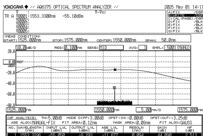
Fig.2: Signal amplification at 1553.33nm @ Pin -55dBm
