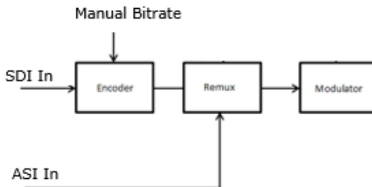
Figure 4.32: Remux work diagram
