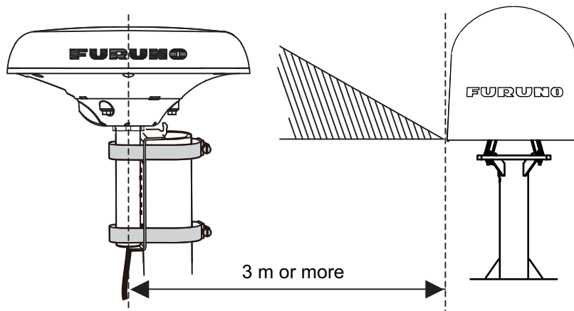
Separation distance from Inmarsat Fleet Broadband Antenna
