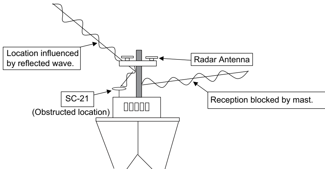
Problems associated with mounting SCX-21 below a radar mast
